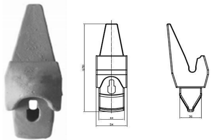
Holder for 18TL Soil Teeth
