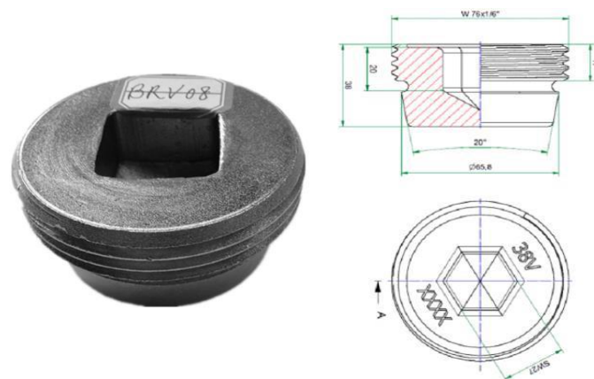
BRV08 Conical bolt for casing
