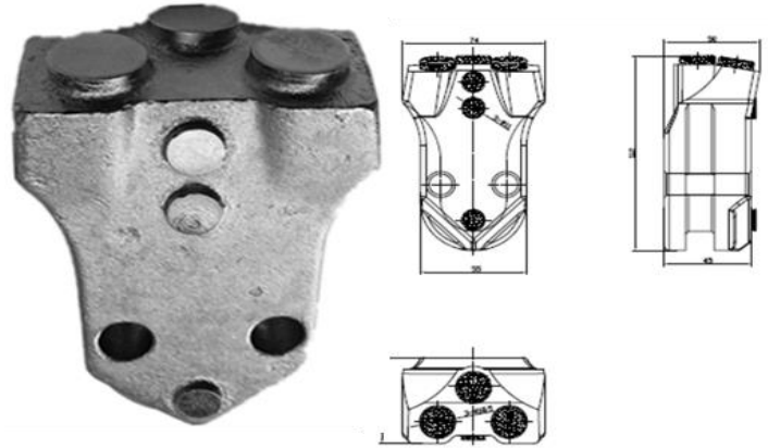
WS46 Casing Teeth
