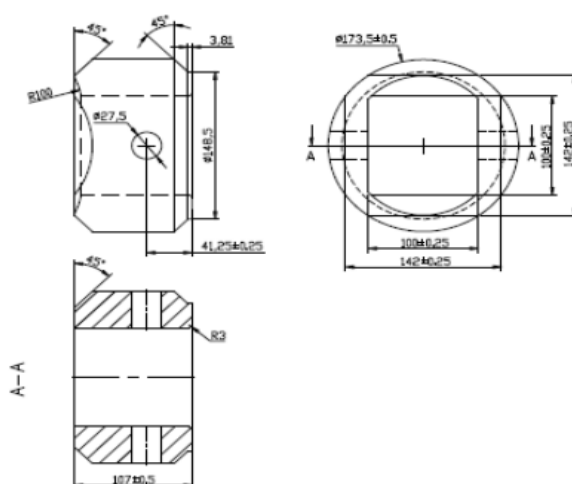
POCKET for FISH TAIL PILOT
