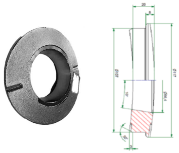
BRV03 Conical ring for casing
